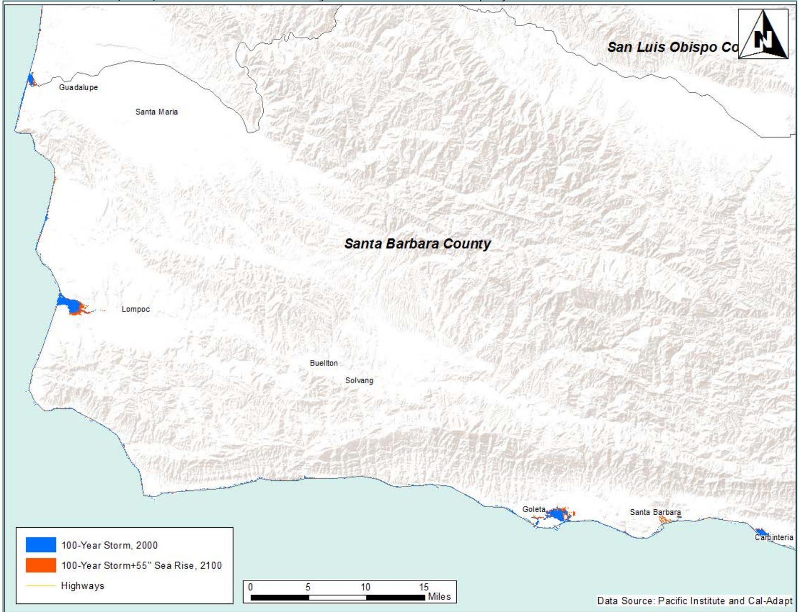
Figure 5. Baseline inundation areas for a 100-year flood (2000) and modeled scenario with additional 55 inches of sea level rise (2100), Santa Barbara County 6 Note: Current SLR projections are 66 inches above sea level. 7
